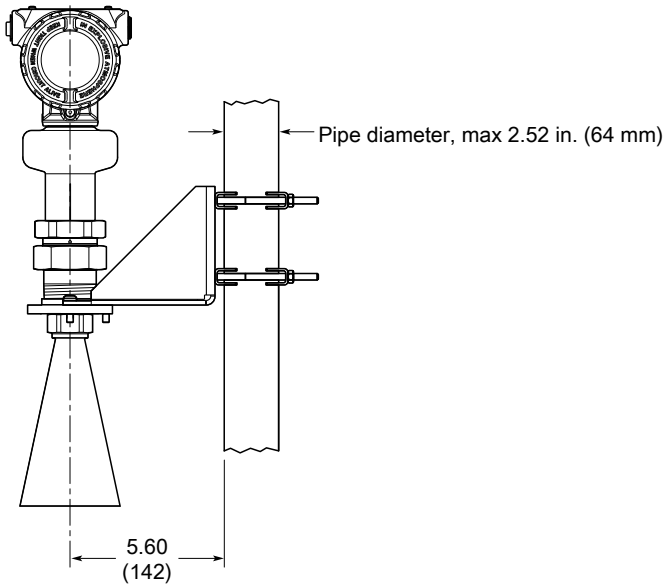
Figure 23: Bracket Mounting (Process Connection Type Code B)
