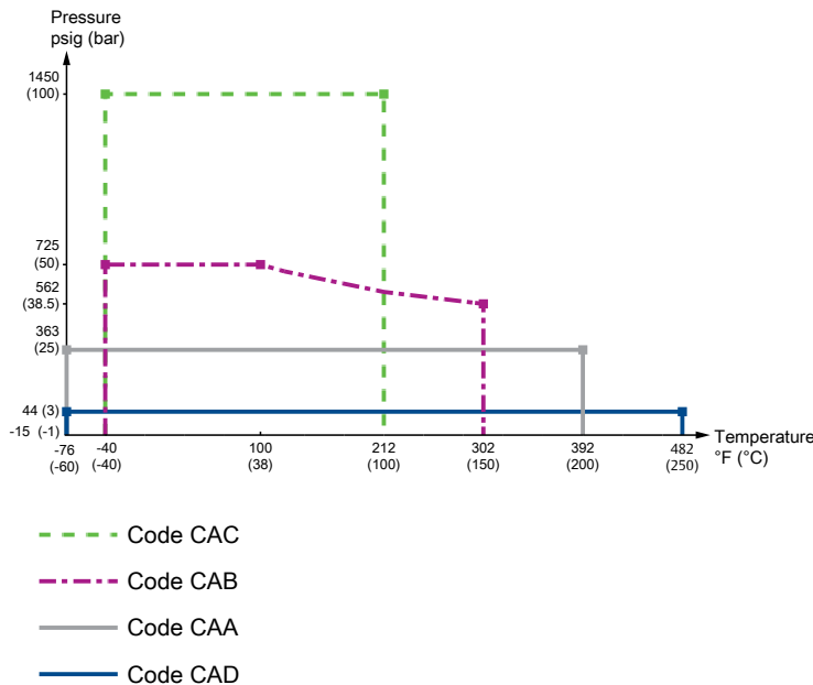
Figure 6: Cone Antenna (PTFE Seal)
