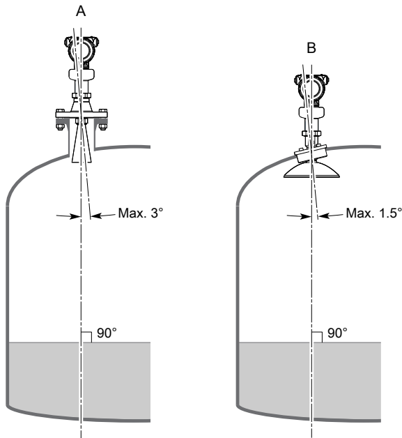
Figure 14: Inclination
