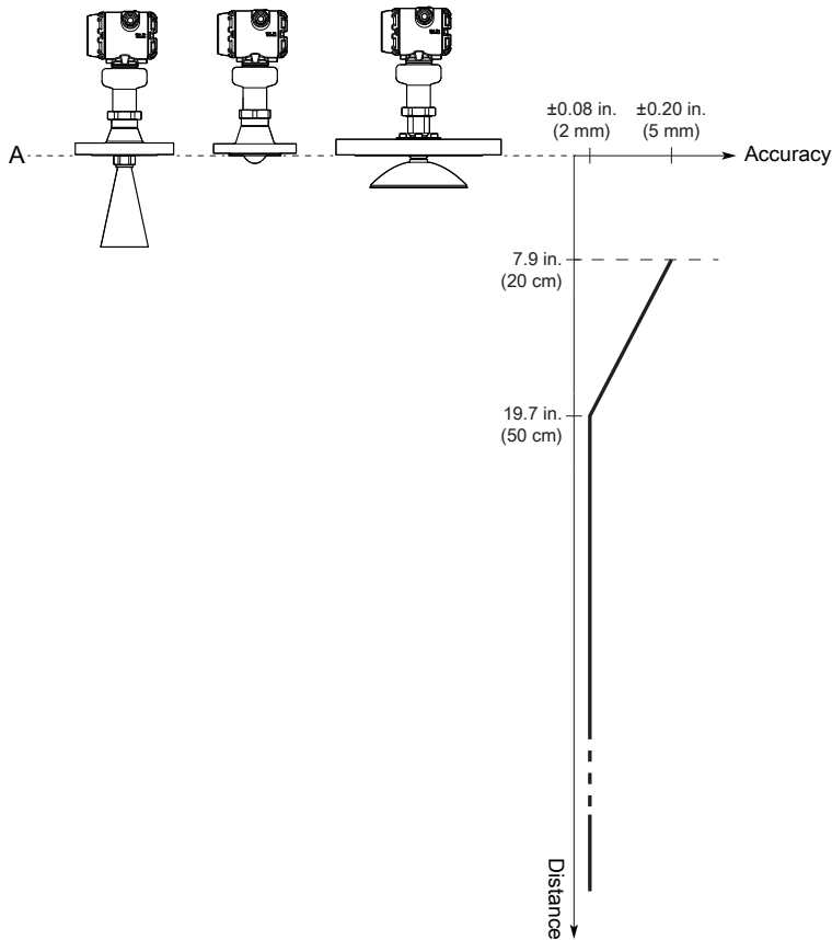
Figure 2: Accuracy Over Measuring Range
