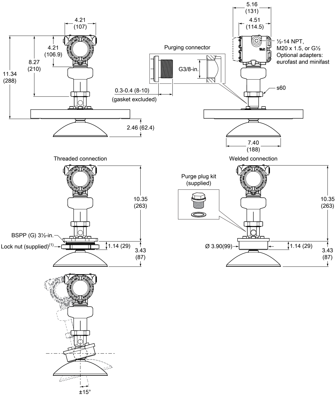
Figure 22: Parabolic Antenna
