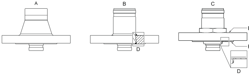
Figure 24: Cone Antenna Flange Connection
