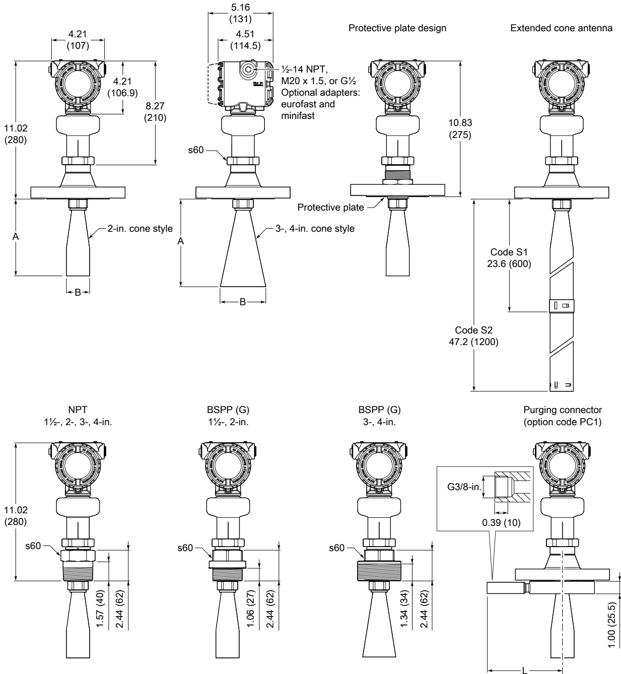
Figure 20: Cone Antenna
