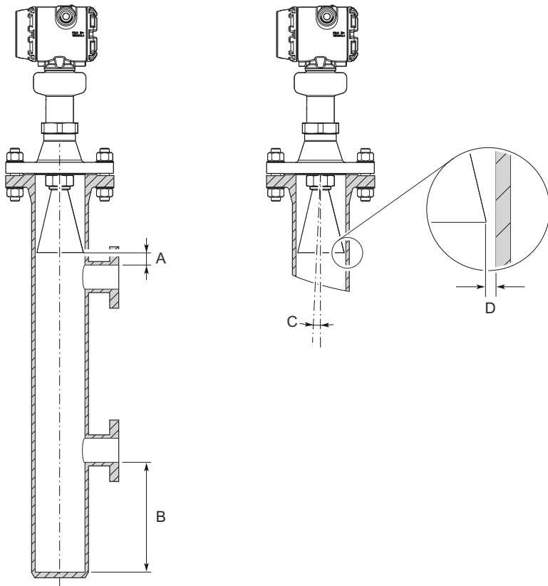
Figure 19: Chamber Requirements
