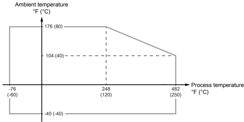
Figure 10: Ambient Temperature vs. Process Temperature
