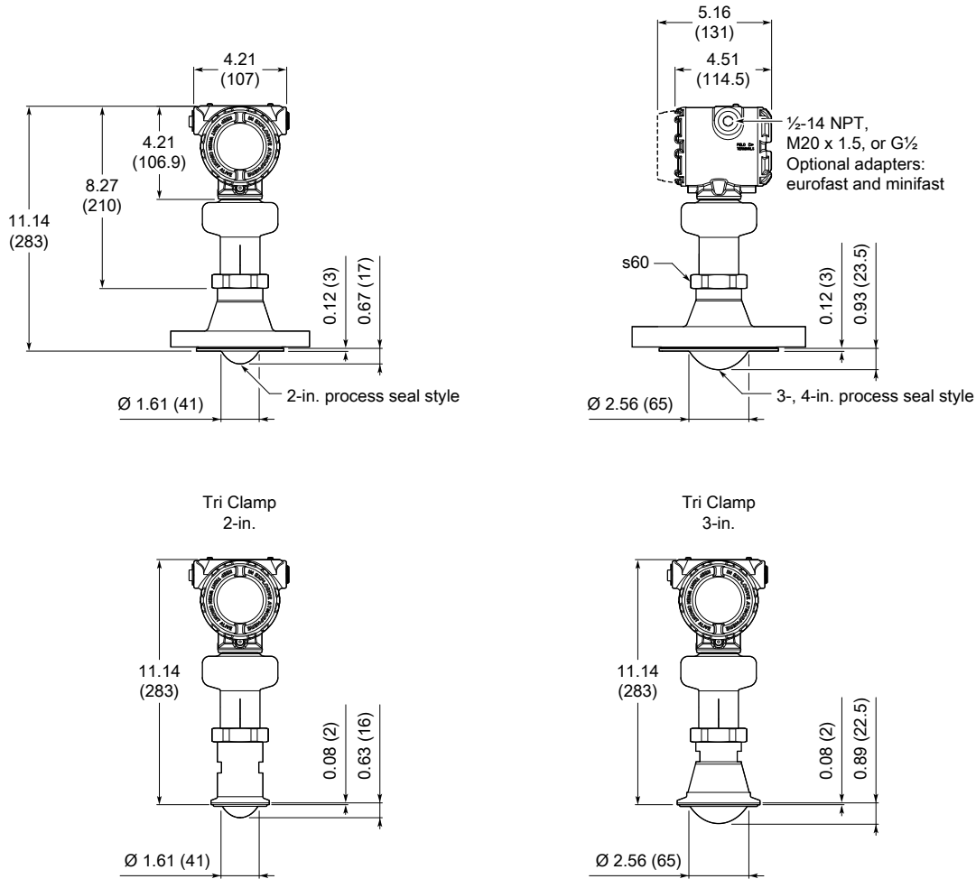
Figure 21: Process Seal Antenna
